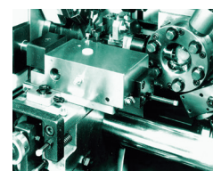
Single point turning attachment
